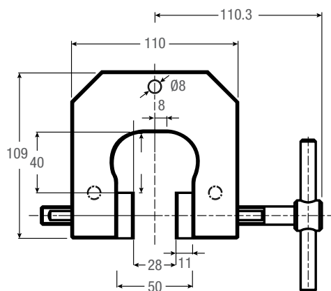
VISE-240G
