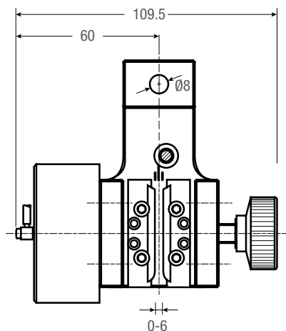
PNEUM-9+KO
