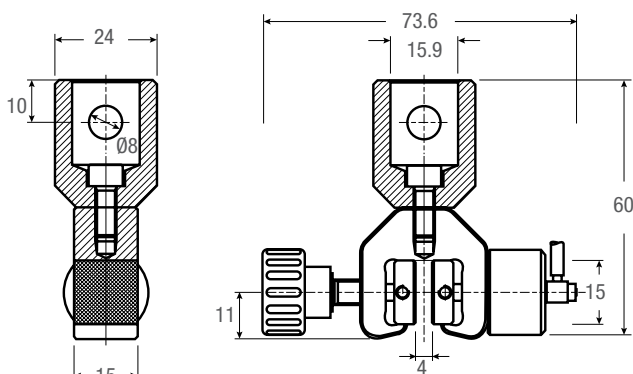
PNEUM-140K+KO
