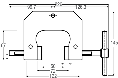
VISE-240G-S50
