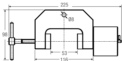
PNEUM-240KA-50-1
