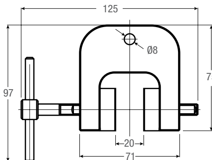
VISE-240KA-20-1
