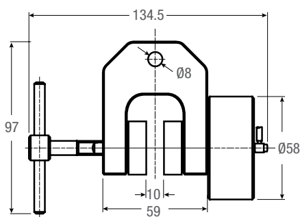
PNEUM-240KA-1
