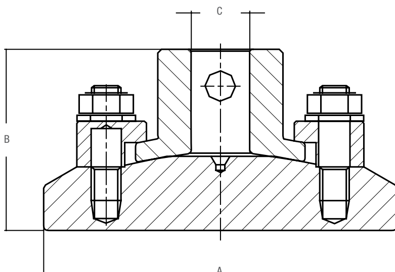
Self-Aligning Circular Platens - Steel
