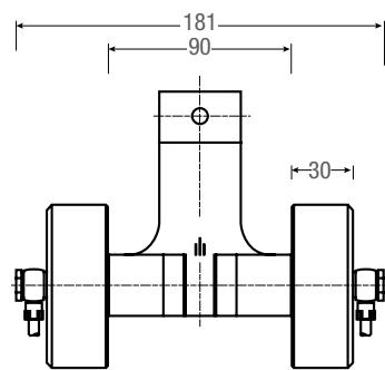
PNEUM-56G2KA-1
