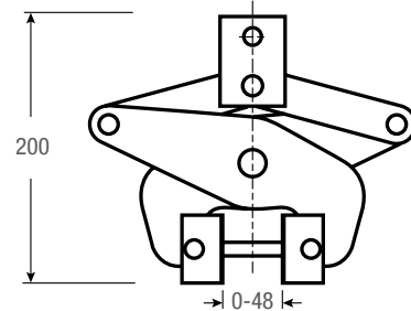
SCISSOR-11-50S-1
