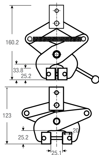
SCISSOR-11-20A-1
