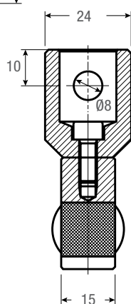
PNEUM-140K+2KO
