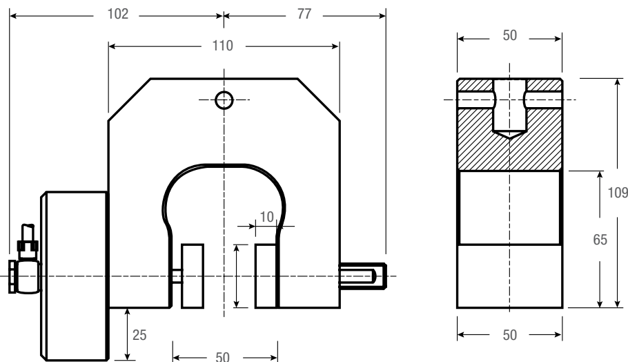
PNEUM-240G+K0
