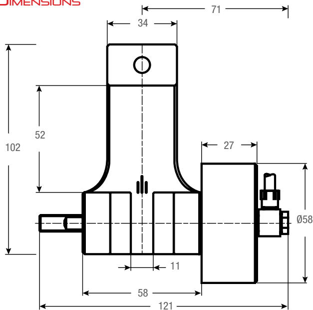
PNEUM-56KA-1
